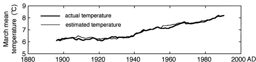
Figure 5. Actual and estimated March mean temperatures during the instrumental period, smoothed by the local linear regression procedure using a 31-year time span.
